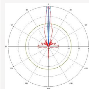
Vertical polarization
