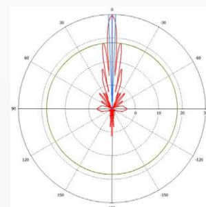
Horizontal polarization
