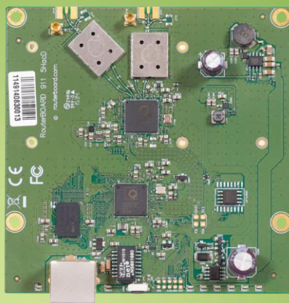
RB911G5-HacD
